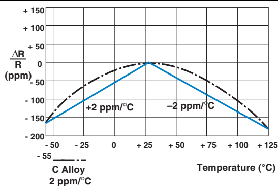
FIGURE 1 - TYPICAL RESISTANCE CHANGE VERSUS TEMPERATURE CURVES AND CHORD SLOPES (TCR) OF TWO ALLOYS IN MILITARY RANGE
