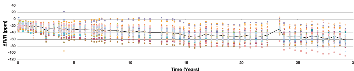
FIGURE 5 - LONG-TERM STABILITY OVER 29 YEARS (0.1W AT 70°C, 50 SAMPLES RCK02, 10KΩ)
