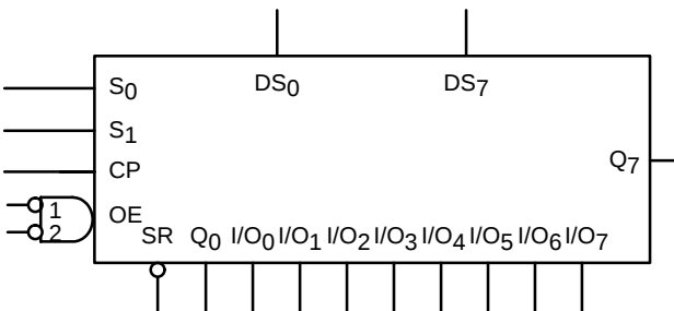
Figure 3. Logic Symbol
