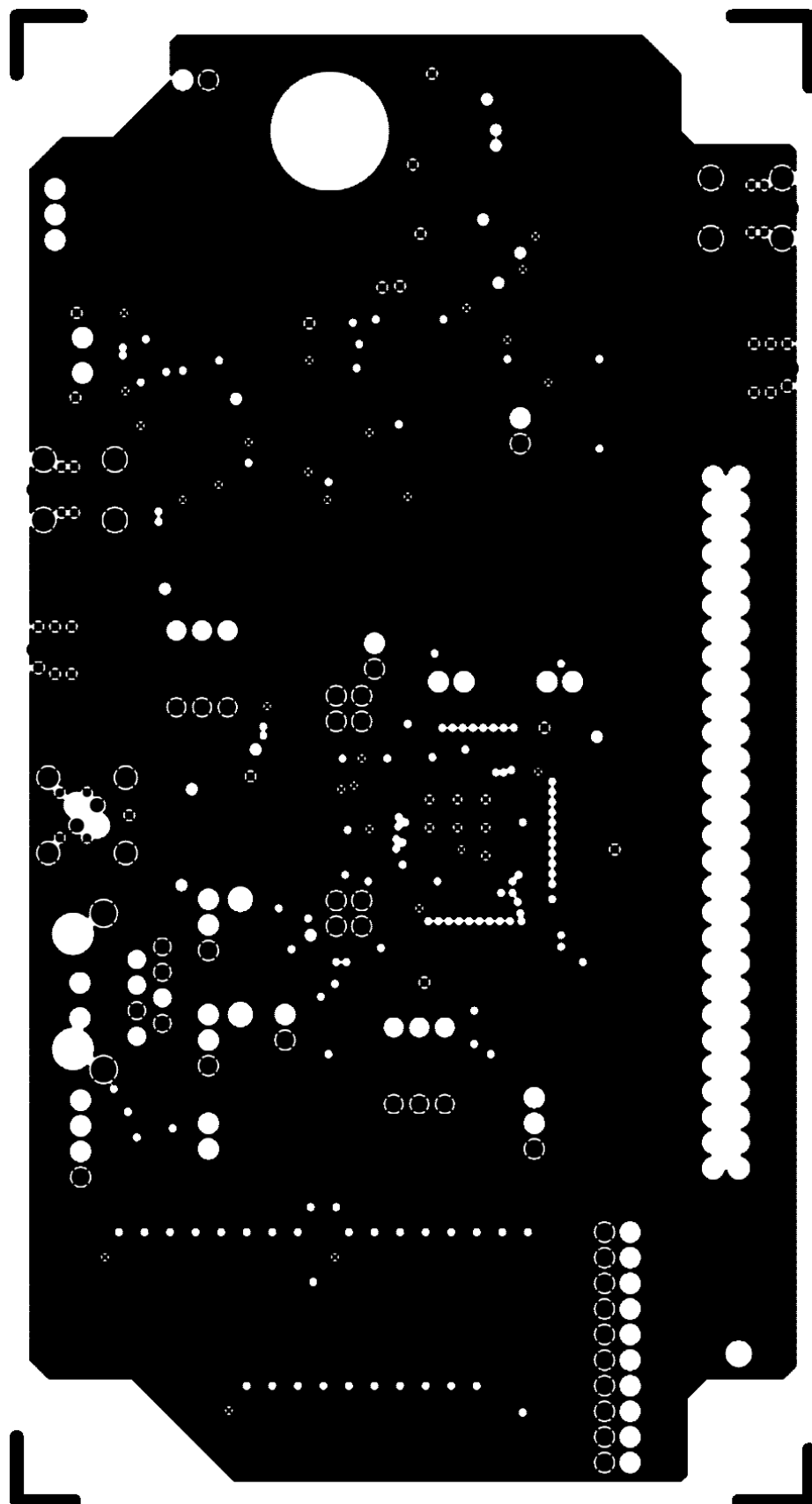
Figure 7: GND Layer
