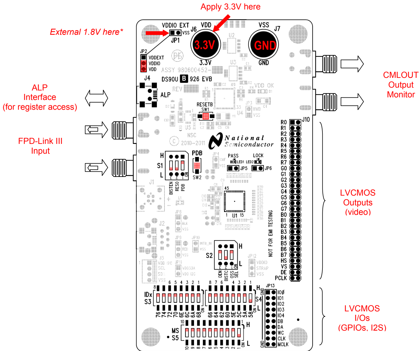
Figure 1: DS90UB926Q EVB
