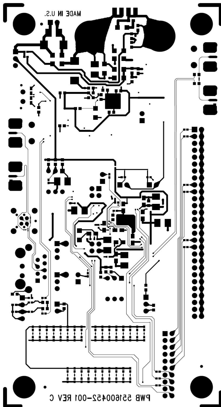
Figure 9: BOTTOM Layer
