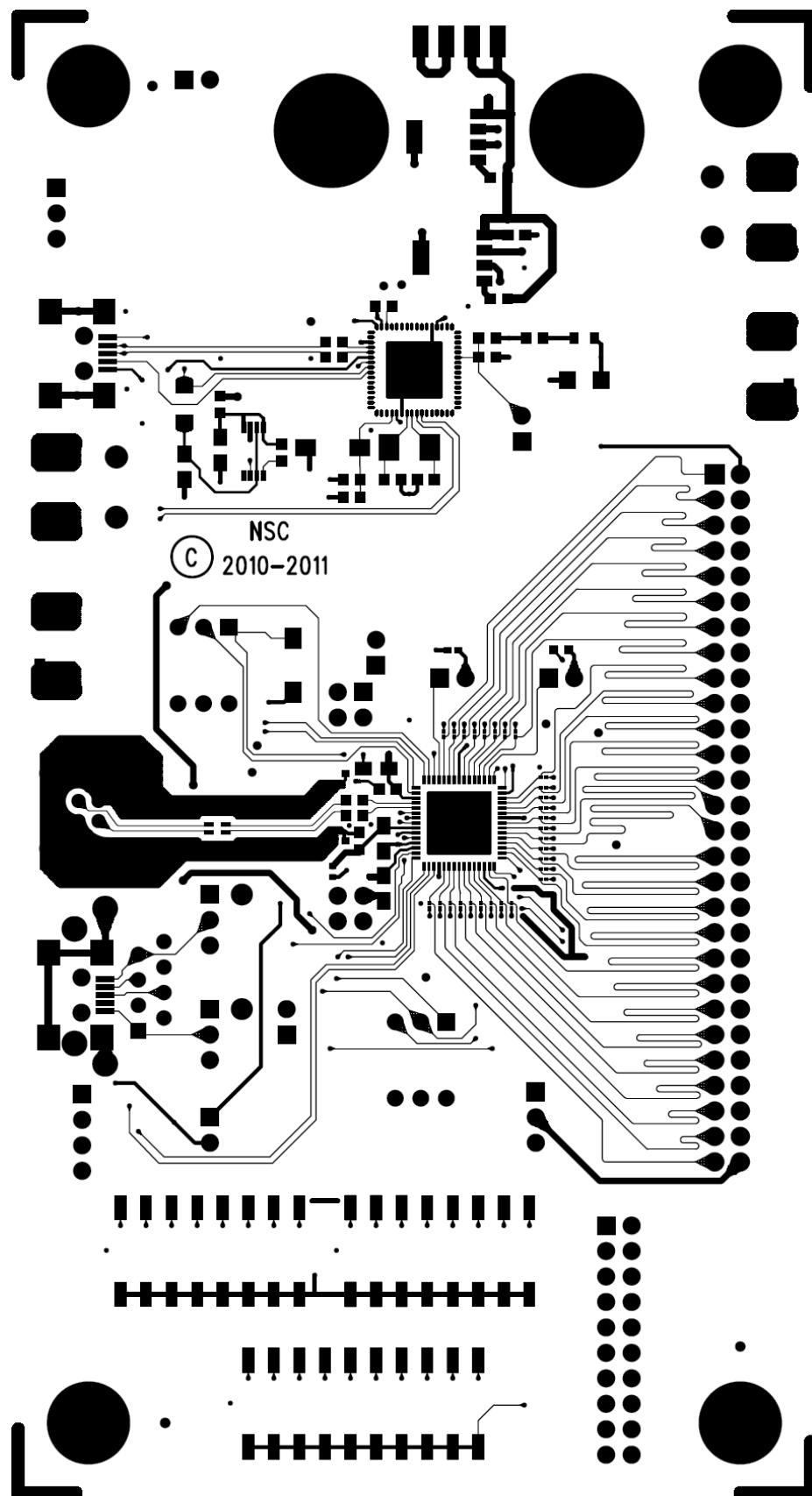
Figure 6: TOP Layer
