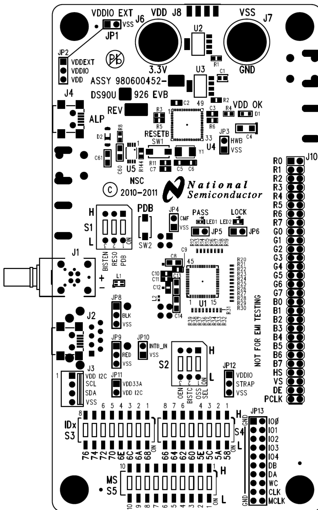
Figure 4: TOP View
