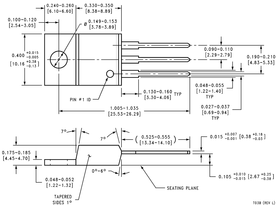
3-Lead TO-220 NS Package Number T03B
