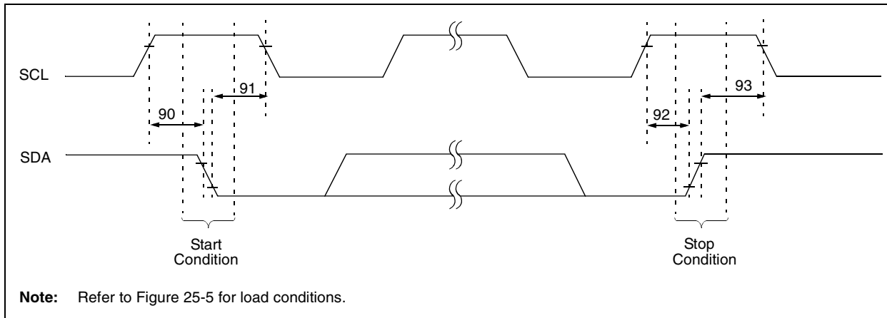
FIGURE 25-19: MASTER SSP I 2 C™ BUS START/STOP BITS TIMING WAVEFORMS
