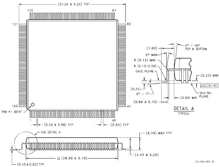
Figure 2: 160-pin EIAJ PQFP mechanical details
