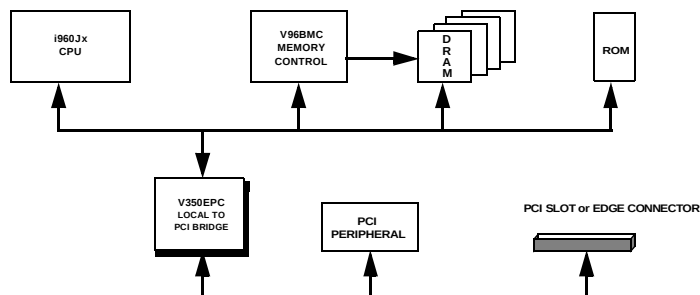
TYPICAL APPLICATION
