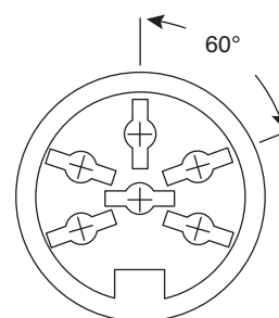
6 Contacts 161-0006-E
