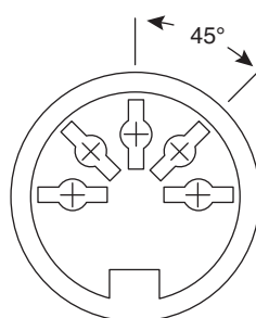
5 Contacts 161-0005-E
