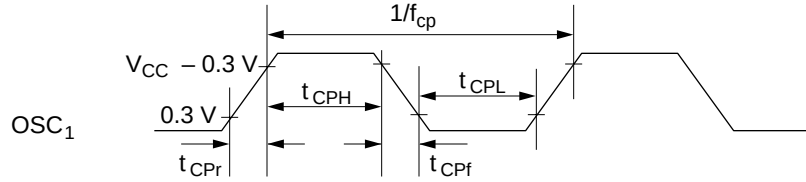
Figure 49 Oscillator Timing
