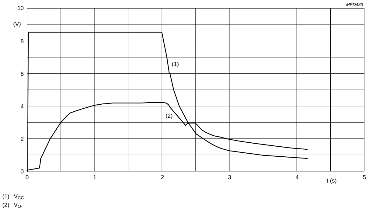
Fig.12 Turn-on/off behaviour.
