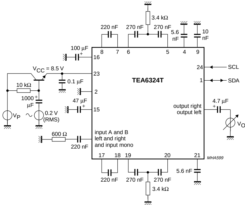
Fig.13 Test circuit for power supply ripple rejection (RR).
