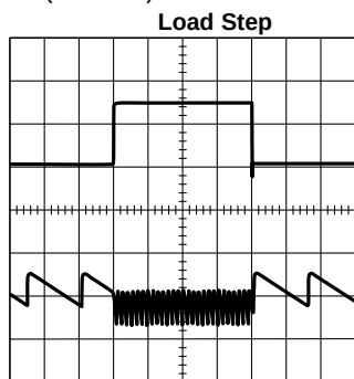
V_{IN} = 3.6V , V_{OUT} = 1.5V , Load = 10mA - 150mA step CH1 (top): Output Current; Scale: 100mA/Div CH2: V_{OUT} ; Scale: 100mV/Div Time scale: 40µs/Div
