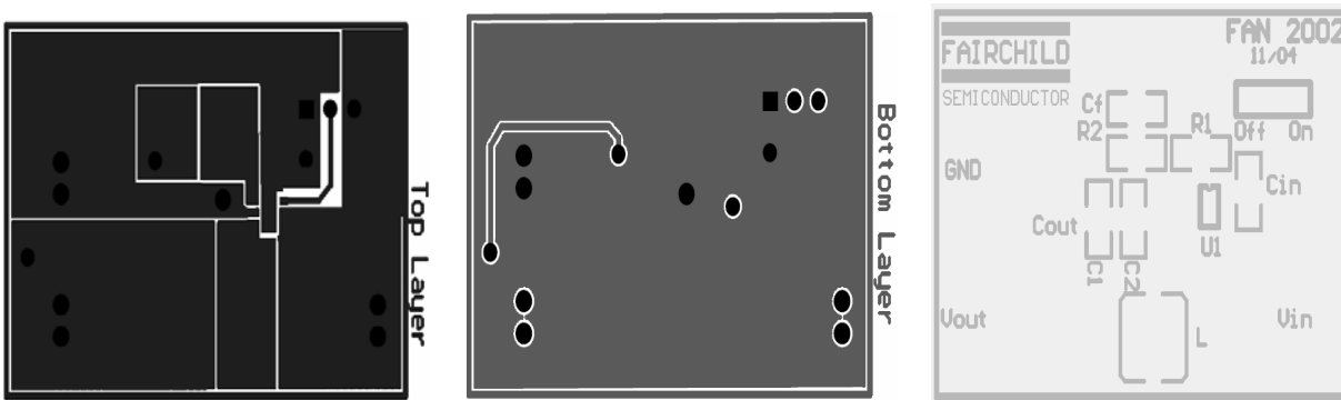
Figure 4. FAN2002MPX PCB Layout
