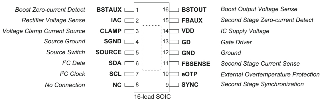
Figure 2. CS1630/31
