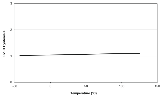
Figure 3. UVLO Characteristics
