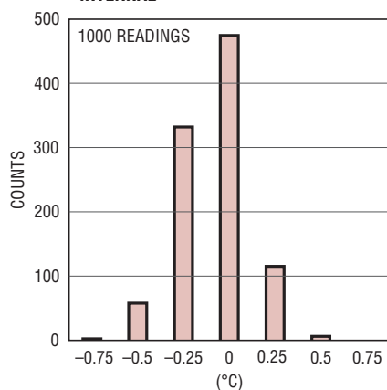
T_{INTERNAL} Noise
