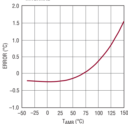
T_{INTERNAL} Error
