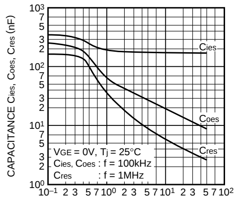
CAPACITANCE VS. V_{CE} (TYPICAL)
