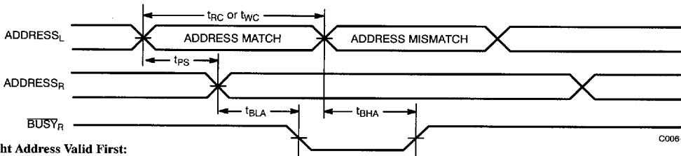
Busy Timing Diagram No. 2 (Address Arbitration) [29]
