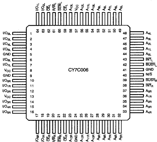
64-Pin TQFP Top View
