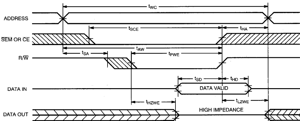
Write Cycle No. 2: R/W Three-State Data I/Os (Either Port) [21, 23, 24]
