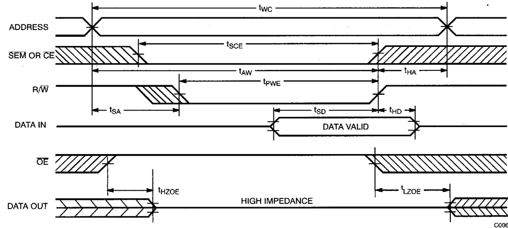
Write Cycle No. 2: R/W Three-State Data I/Os (Either Port) [21, 23, 24]
