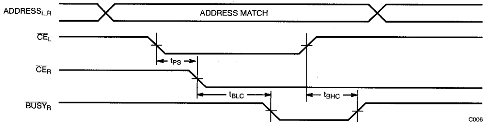
Busy Timing Diagram No. 1 ( \overline{CE} Arbitration) [29]
