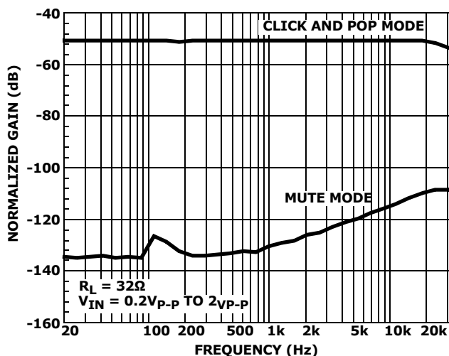
FIGURE 14. OFF-ISOLATION
