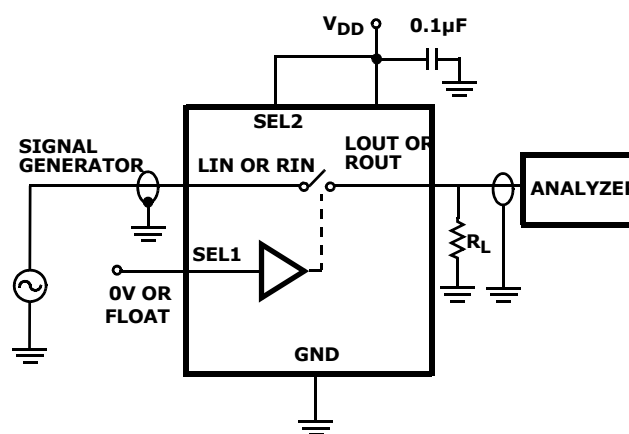
FIGURE 3. OFF ISOLATION CIRCUIT
