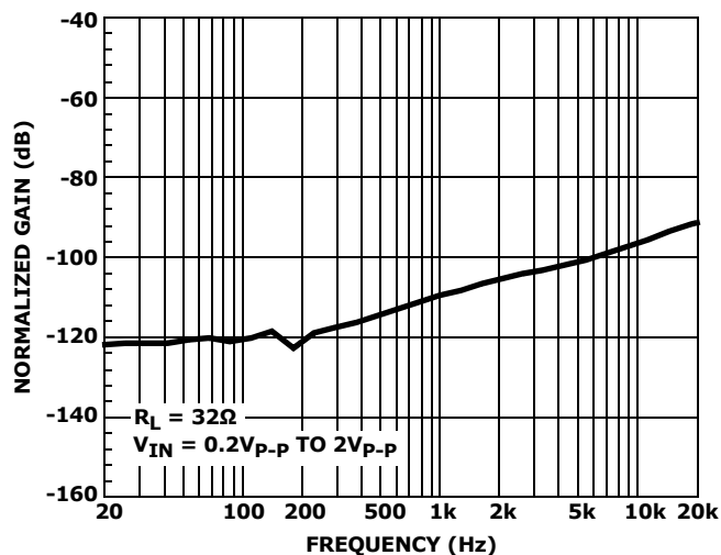
FIGURE 15. CROSSTALK
