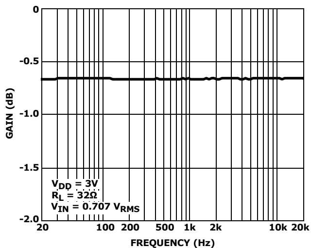
FIGURE 13. INSERTION LOSS
