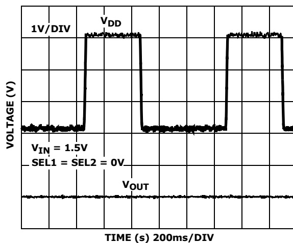
FIGURE 16. POWER-UP/POWER-DOWN CLICK AND POP TRANSIENT
