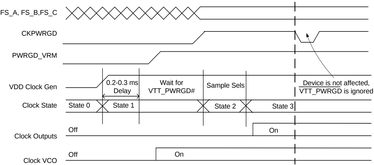
Figure 3. CKPWRGD Timing Diagram
