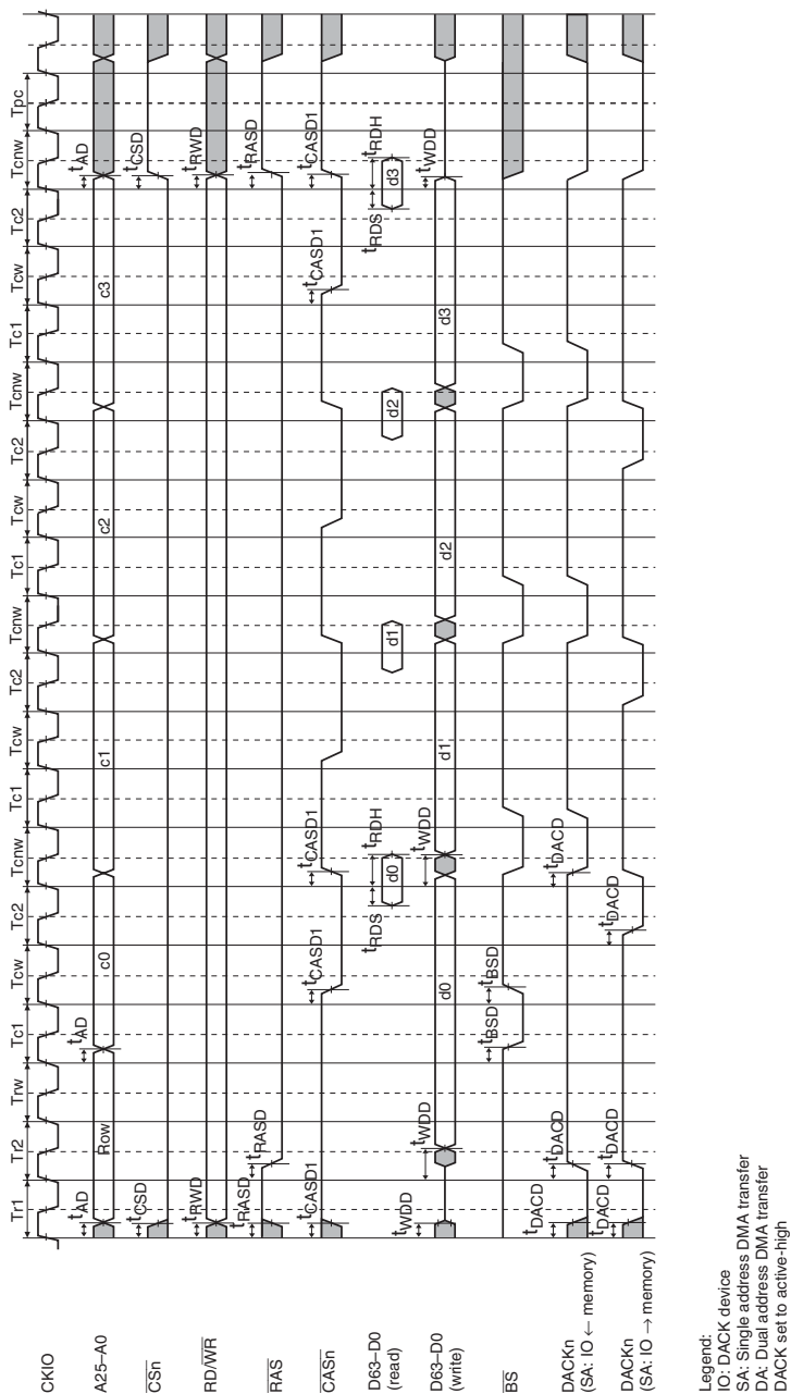
Figure 22.46 DRAM Burst Bus Cycle (Fast Page Mode, RCD[1:0] = 01, AnW[2:0] = 001, TPC[2:0] = 001, 2-Cycle CAS Negate Pulse Width)
