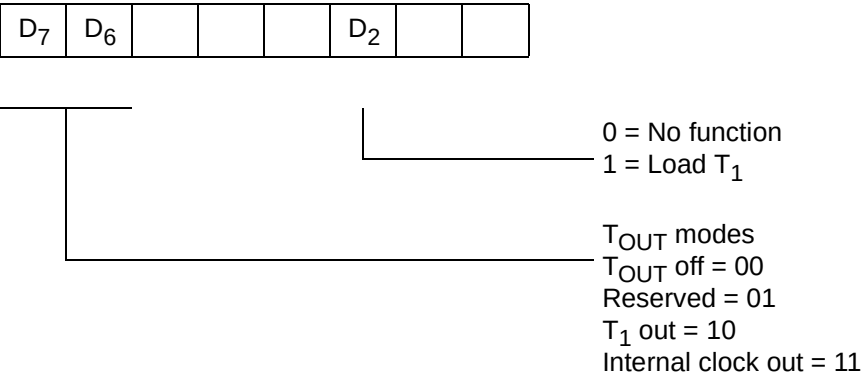
Figure 25. Timer Mode Register T OUT Operation
