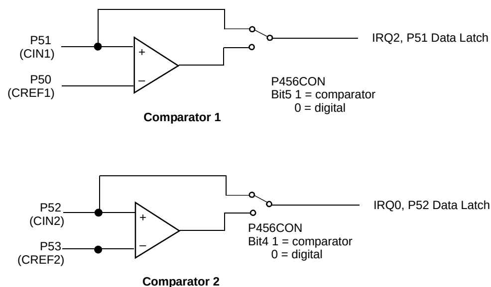
Figure 13. Analog Comparators
