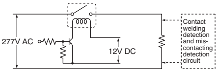
4. Electrical life test (5 A 277 V AC, resistive load) Sample: ALTS3125, 6 pcs. Operation frequency: 20 times/min. (ON/OFF = 1.5s: 1.5s) Ambient temperature: 20°C 68°F
