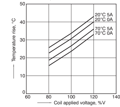
2. Coil temperature rise Sample: ALTS3125, 6 pcs. Point measured: coil inside Contact current: 0 A, 5A
