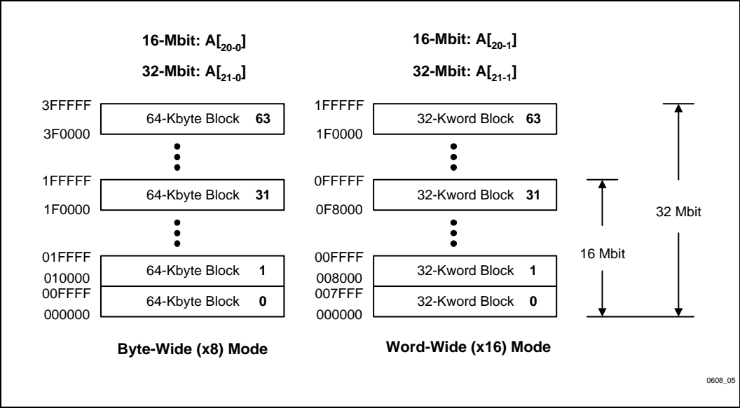
Figure 4. Memory Map
