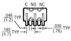
1 Pole P.C. Mounting
