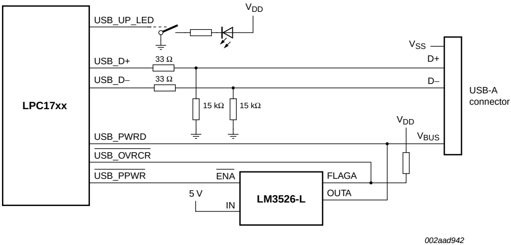
Fig 32. USB host port configuration
