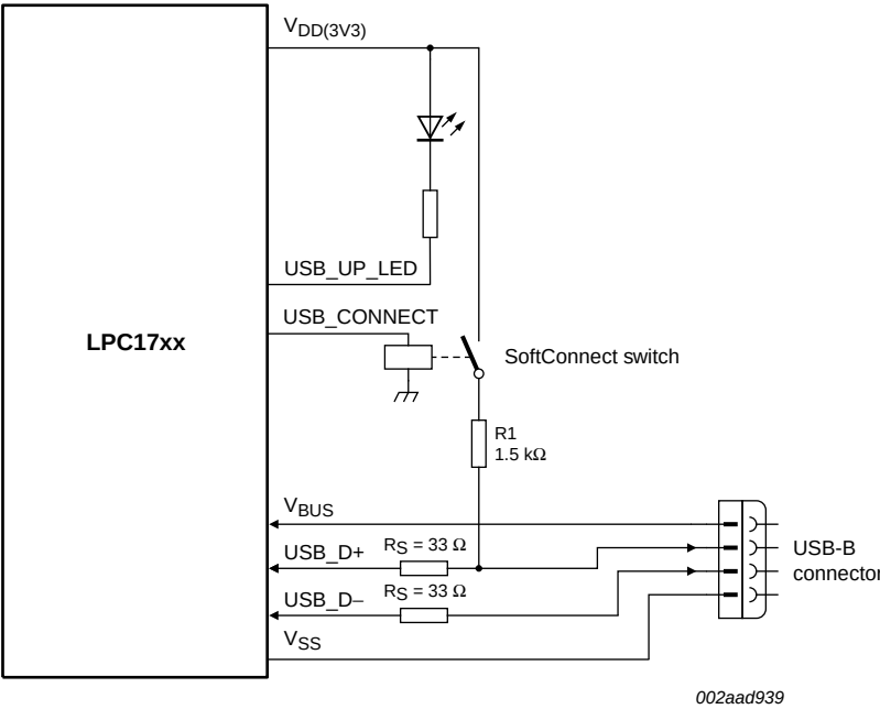
Fig 30. USB interface with soft-connect
