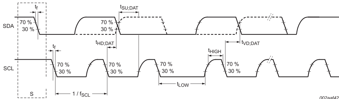
Fig 17. I 2 C-bus pins clock timing
