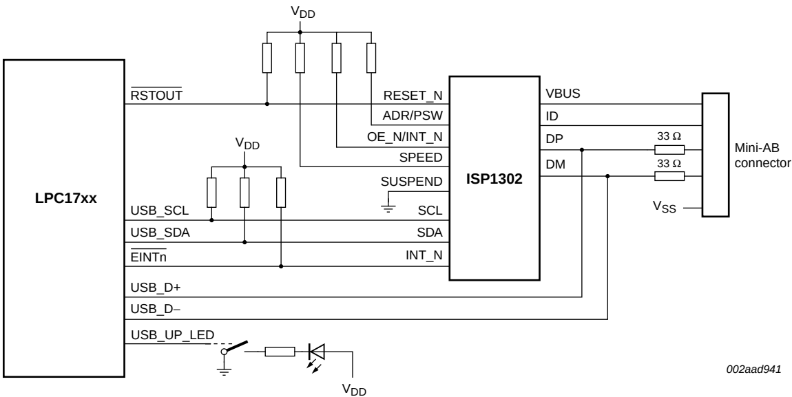
Fig 31. USB OTG port configuration
