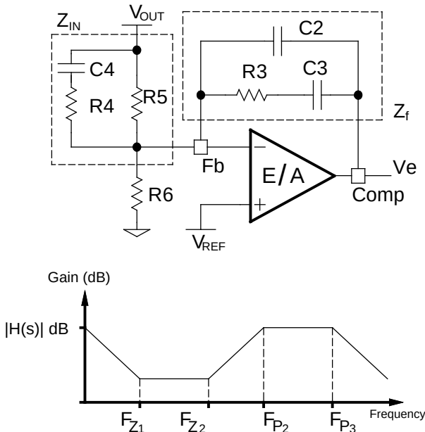
Figure 34: Type III Compensation network and its asymptotic gain plot
