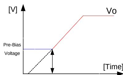
Figure 8: Pre-Bias startup
