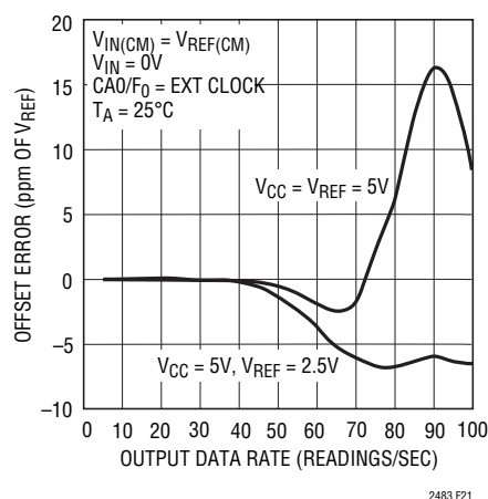
Figure 21. Offset Error vs Output Data Rate and Reference Voltage
