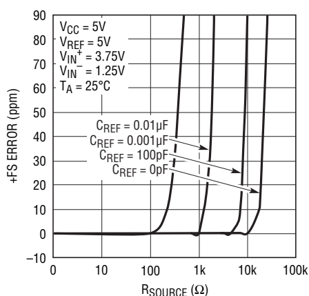
Figure 11. +\text{FS} Error vs R_{\text{SOURCE}} at \text{REF}^+ or \text{REF}^- (Small C_{\text{REF}} )
