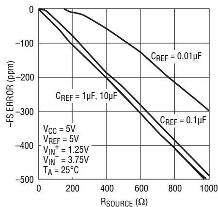
Figure 14. -\text{FS} Error vs R_{\text{SOURCE}} at \text{REF}^+ or \text{REF}^- (Large C_{\text{REF}} )
