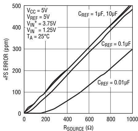
Figure 13. +\text{FS} Error vs R_{\text{SOURCE}} at \text{REF}^+ or \text{REF}^- (Large C_{\text{REF}} )
