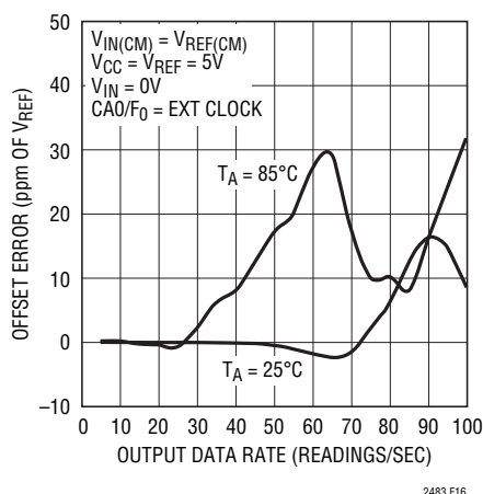
Figure 16. Offset Error vs Output Data Rate and Temperature
