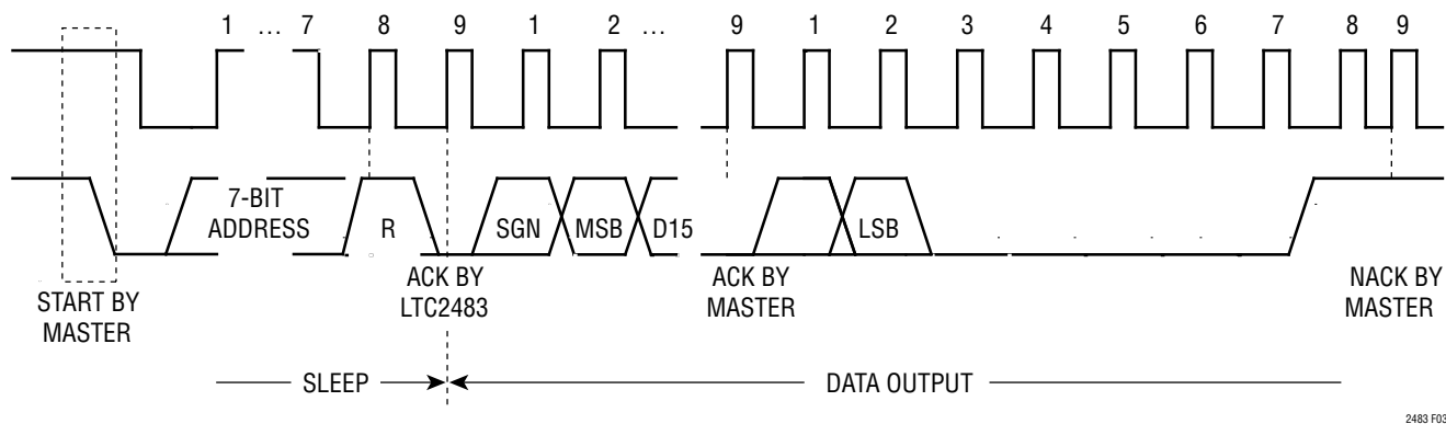
Figure 3. Timing Diagram for Reading from the LTC2483
