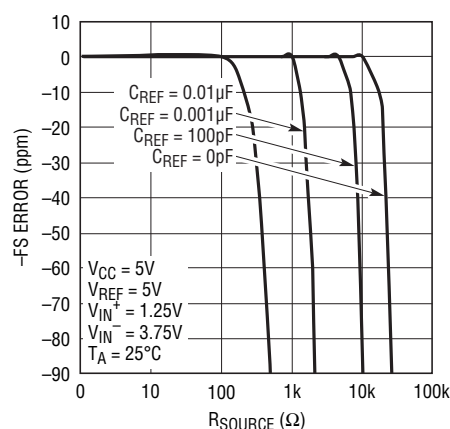
Figure 12. -\text{FS} Error vs R_{\text{SOURCE}} at \text{REF}^+ or \text{REF}^- (Small C_{\text{REF}} )
