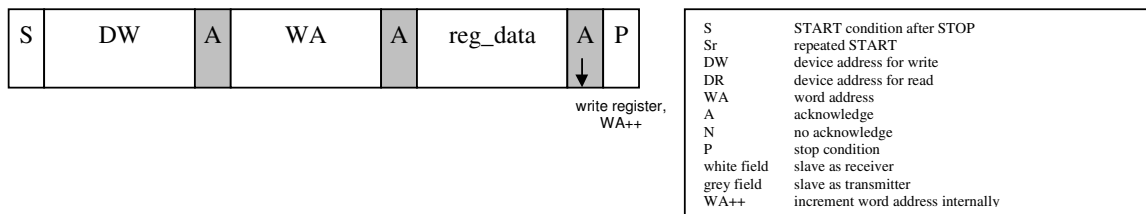
Figure 1 – I^2C Byte-Write:
