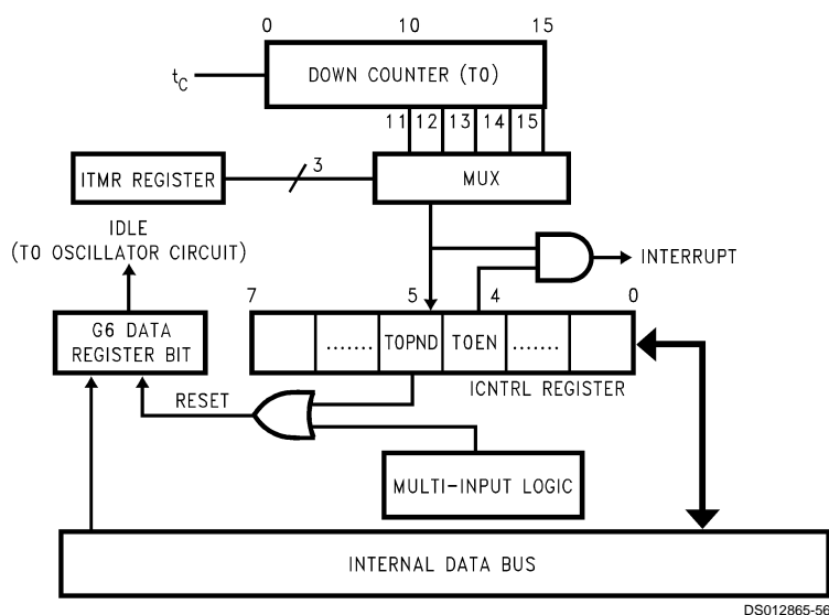
FIGURE 8. Functional Block Diagram for Idle Timer T0
