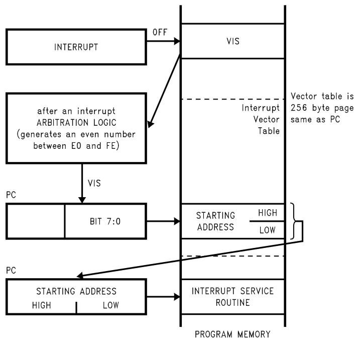
FIGURE 16. VIS Flowchart
