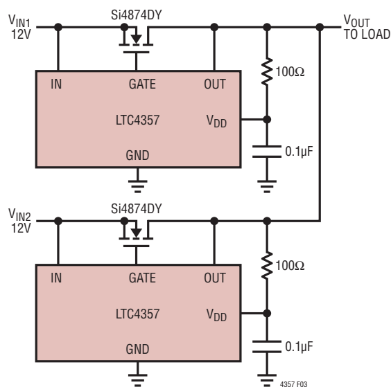
Figure 3. 12V, 10A Diode-OR
