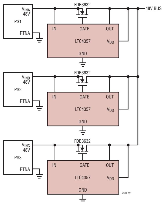
Figure 1. Droop Sharing Redundant Supplies
