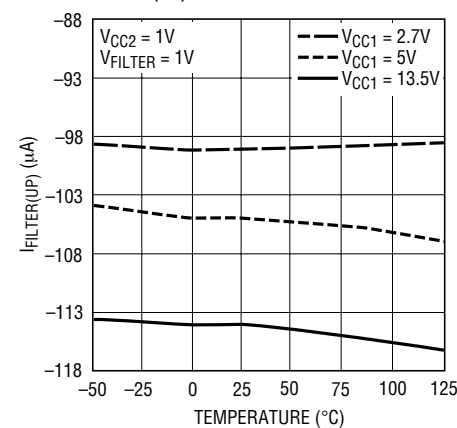
I_{FILTER(UP)} vs Temperature
