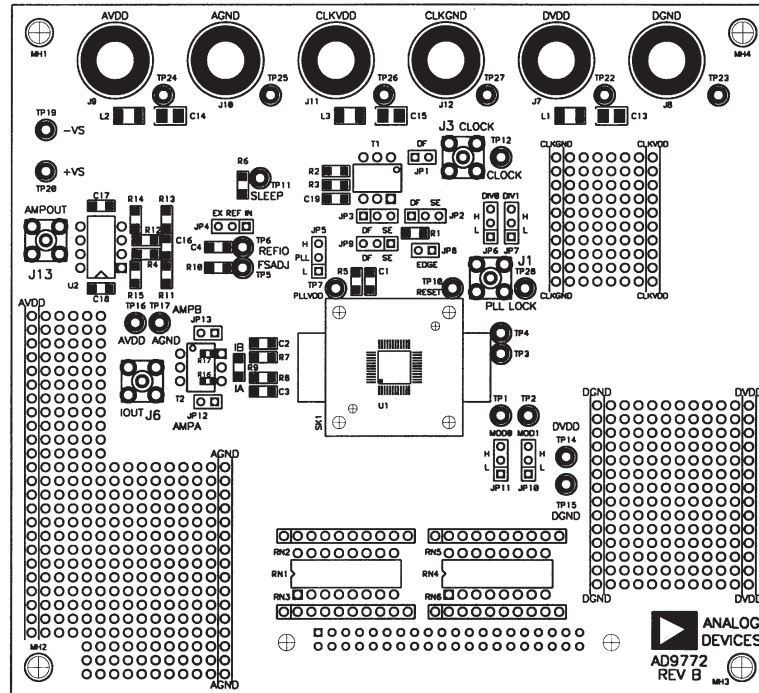
Figure 39. Silkscreen Layer—Top
