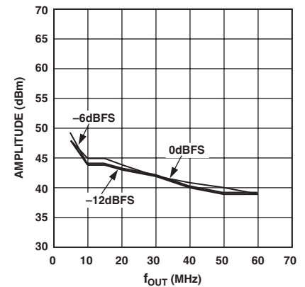
TPC 9. Out-of-Band SFDR vs. f_{OUT} @ f_{DATA} = 160 MSPS
