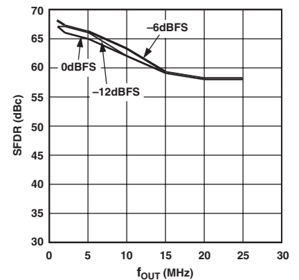
TPC 3. Out-of-Band SFDR vs. f_{OUT} @ f_{DATA} = 65 MSPS
