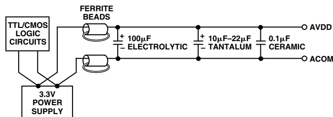
Figure 29. Differential LC Filter for 3.3 V
