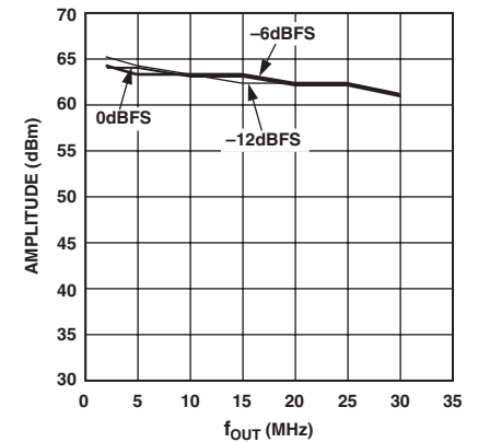
TPC 6. Out-of-Band SFDR vs. f_{OUT} @ f_{DATA} = 78 MSPS
