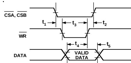
Figure 3. AD7847 Write Cycle Timing Diagram
