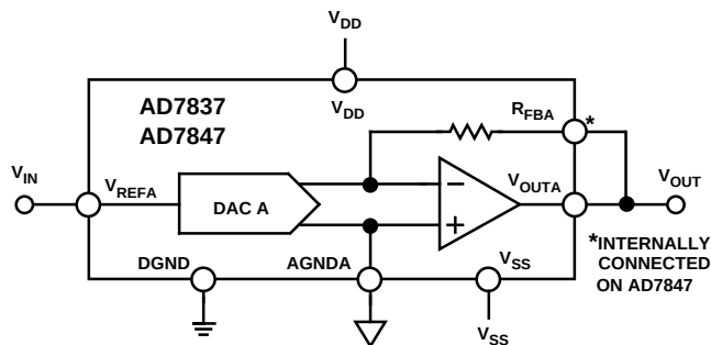
Figure 6. Unipolar Binary Operation
