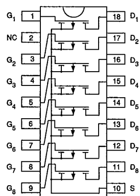
top view 18-pin DIP
