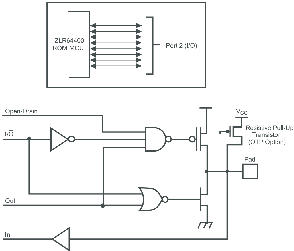
Figure 5. Port 2 Configuration
