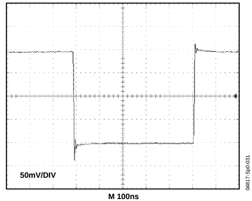
Figure 14. Small Signal Pulse Response R_{LOAD} = 1 \text{ k}\Omega , R_{FB} = 500 \Omega
