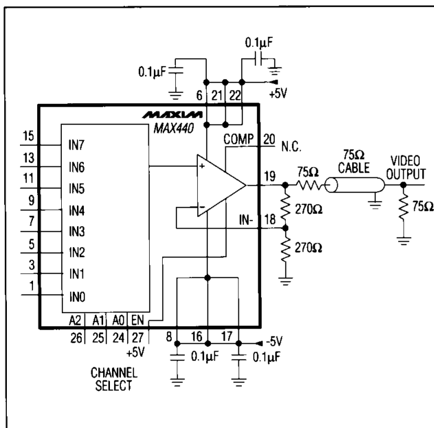
Capacitive-Load Driving
