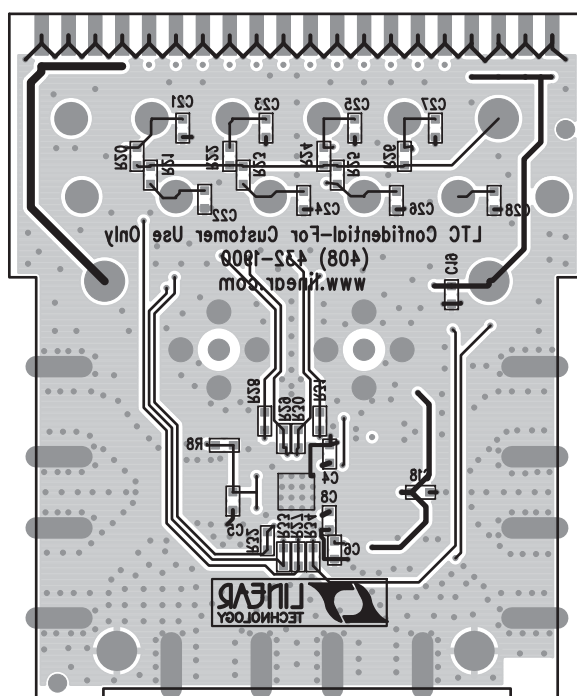
Figure 27. Silkscreen Bottom
