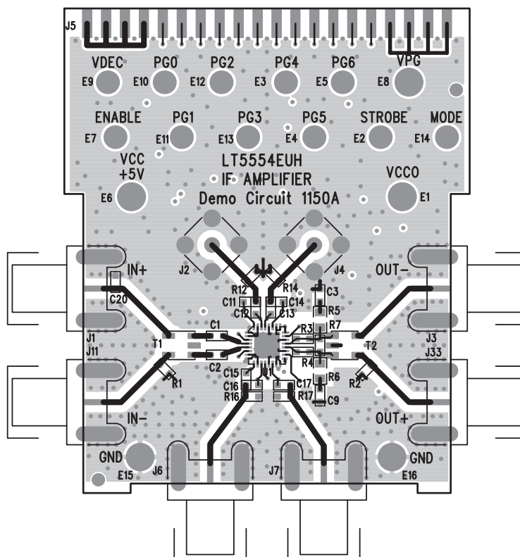
Figure 26. Silkscreen Top
