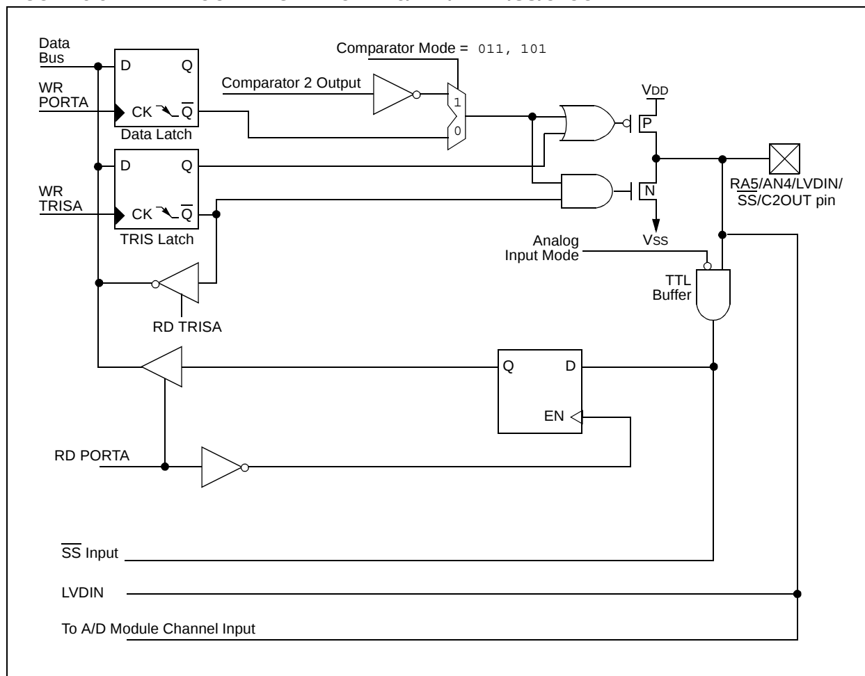
FIGURE 5-5: BLOCK DIAGRAM OF RA5/AN4/LVDIN/ \overline{\text{SS}} /C2OUT PIN
