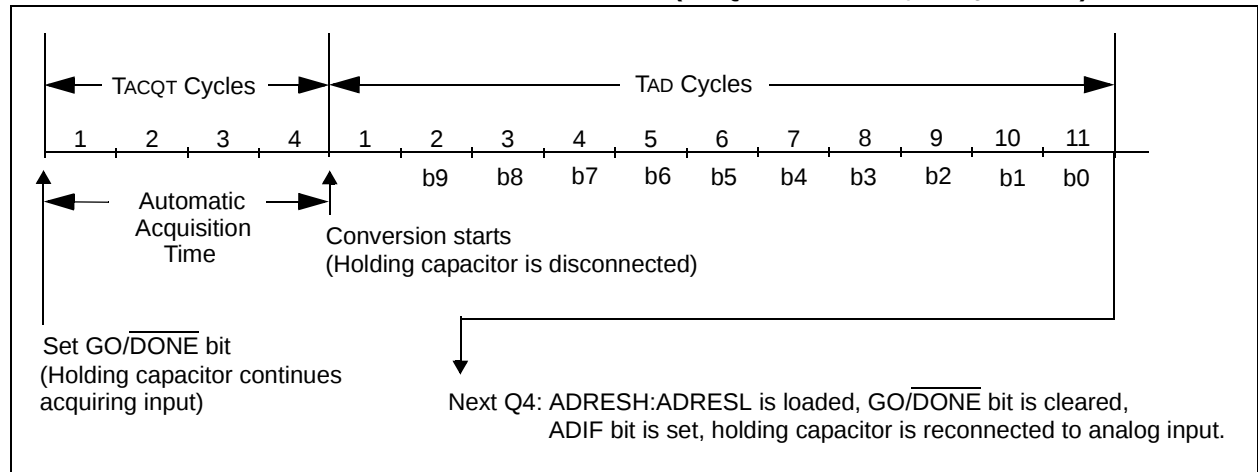
FIGURE 12-4: A/D CONVERSION TAD CYCLES (ACQT<2:0> = 010, Tacq = 4 TAD)
