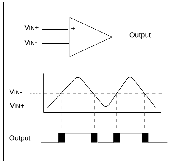
FIGURE 13-2: SINGLE COMPARATOR
