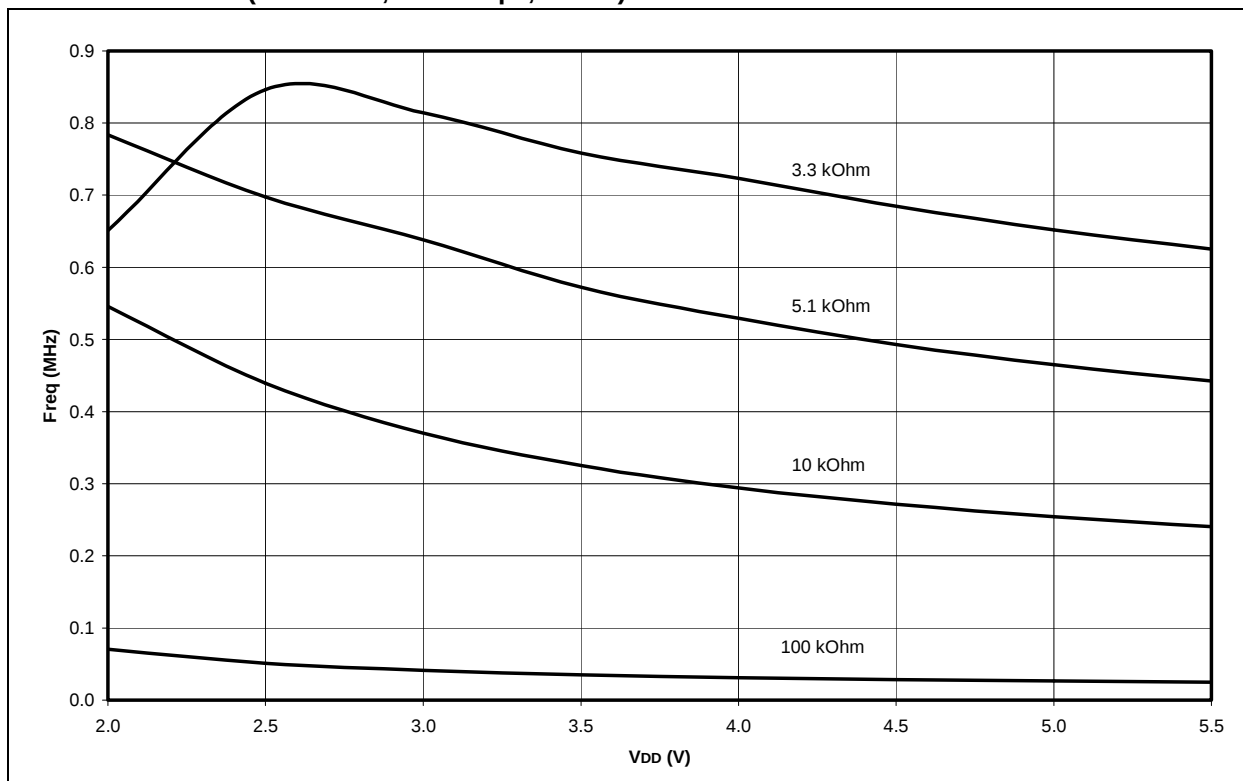
FIGURE 19-13: AVERAGE F_{osc} vs. V_{DD} FOR VARIOUS VALUES OF R (RC MODE, C = 300\text{ pF} , +25^\circ\text{C} )
