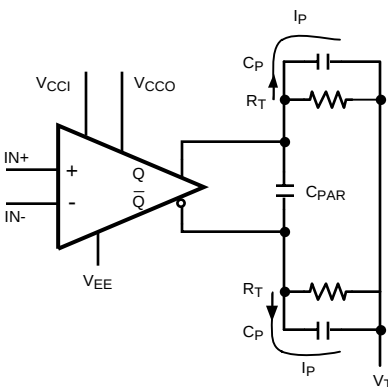
Figure 30. Parasitic Capacities
