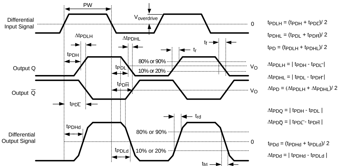
Figure 15. Timing Definitions
