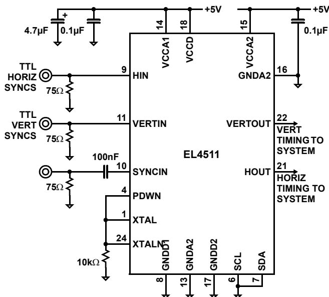
FIGURE 8. APPLICATIONS DRAWING 1
