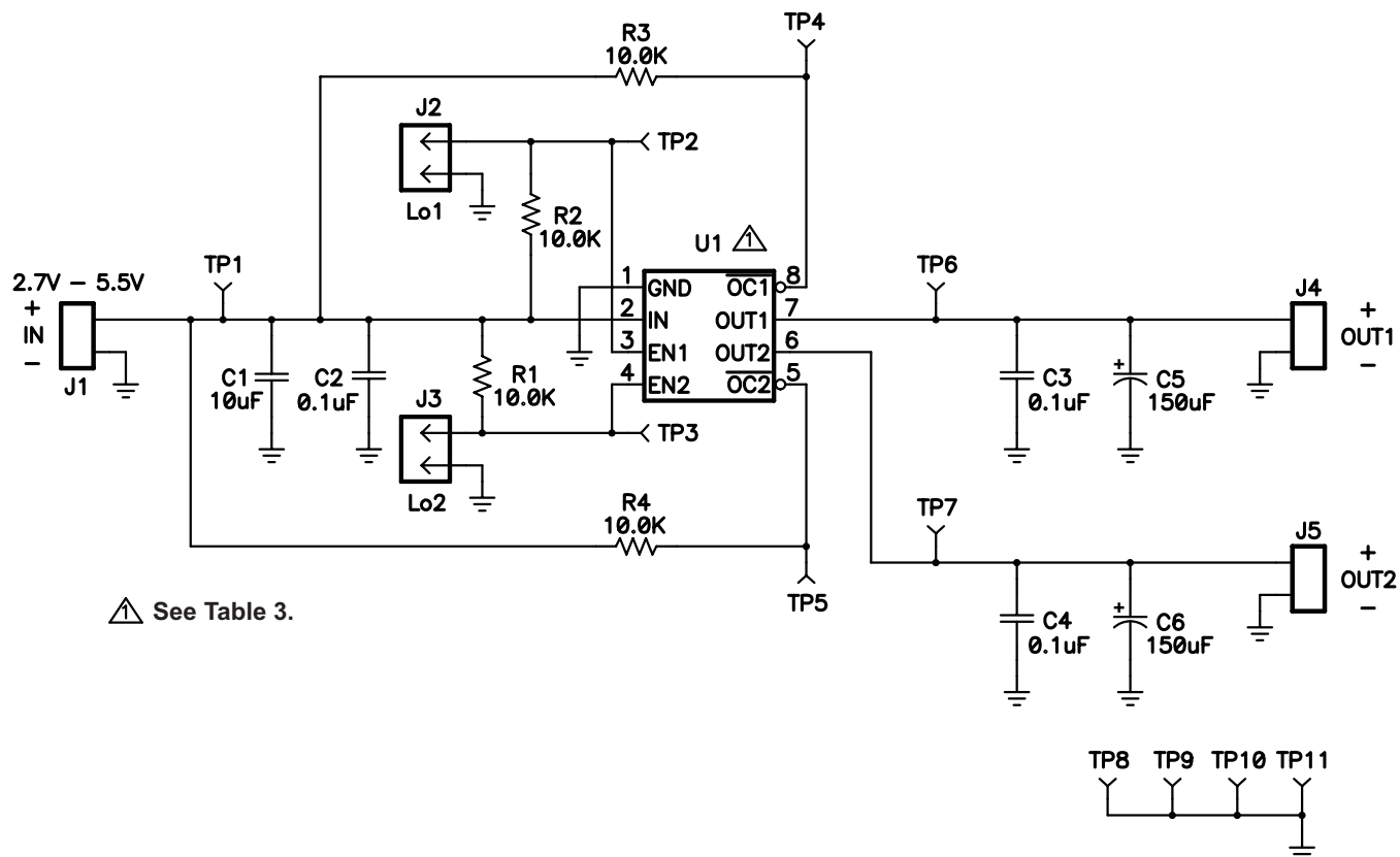
Figure 1. TPS20xxEVM-293 Schematic
