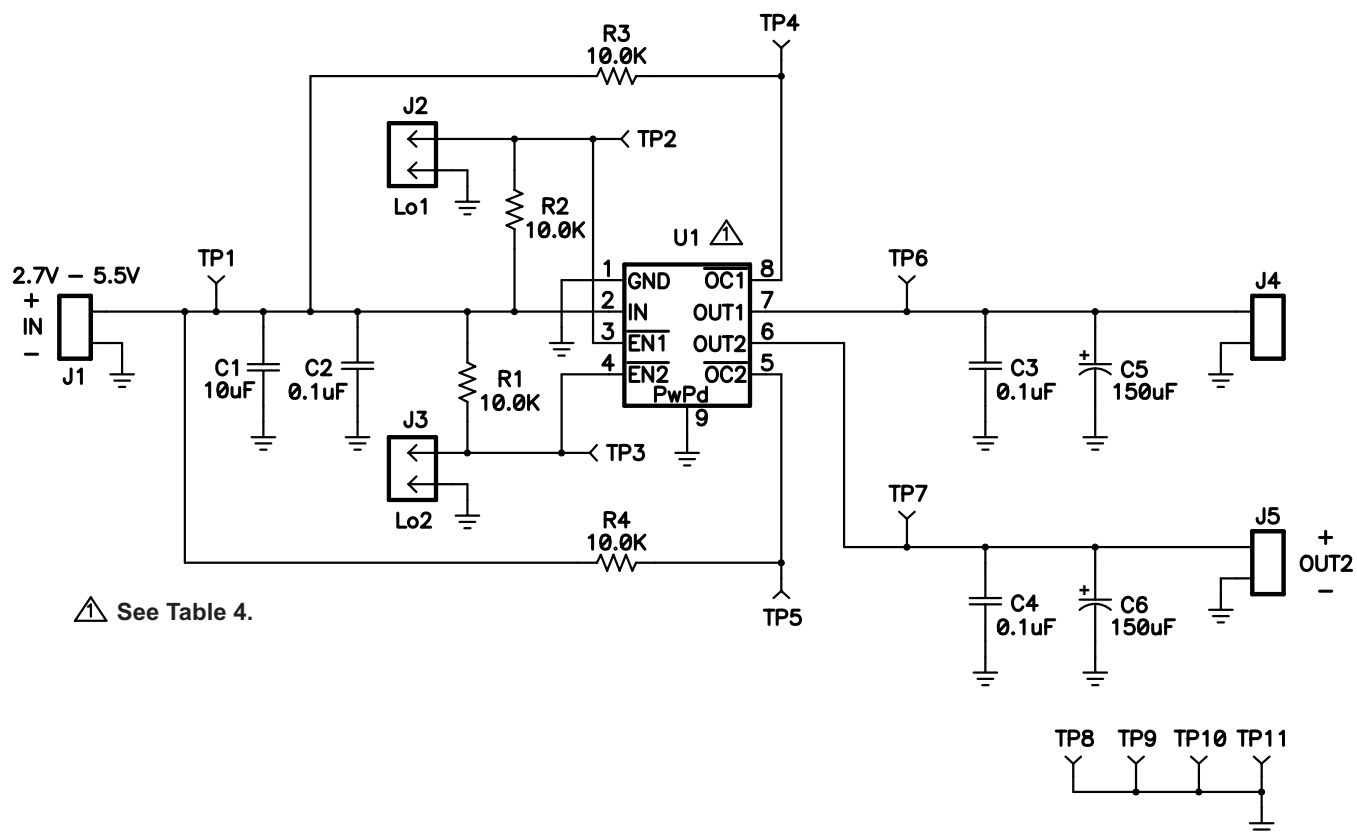
Figure 2. TPS20xxEVM-296 Schematic
