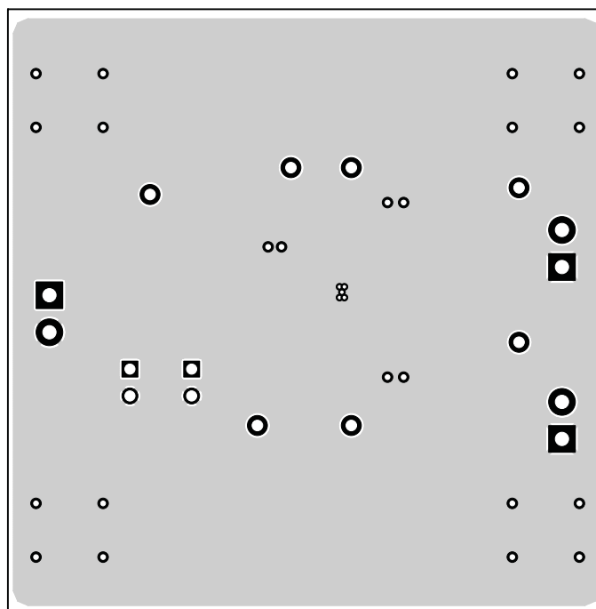
Figure 8. TPS20xxEVM-296 Bottom-Side Layout
