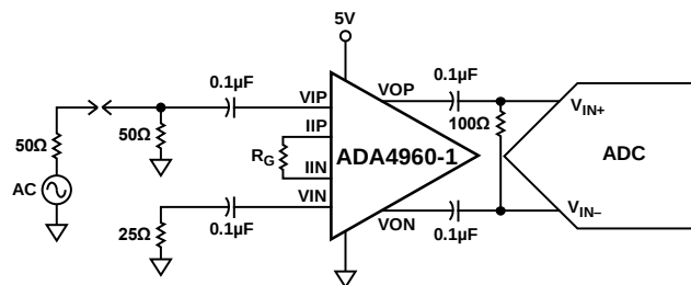
Figure 41. Single-Ended Input Configuration, AC-Coupled to the ADC
