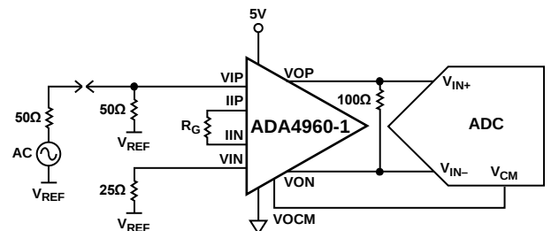
Figure 40. Single-Ended Input Configuration, DC-Coupled Inputs and Outputs
