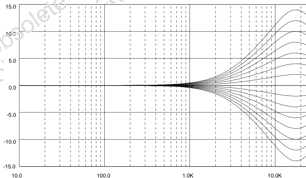
Figure 15. Treble Control @ f_C = 17.5kHz
