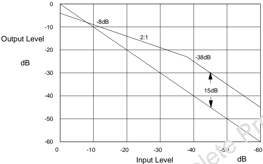
Figure 22. Compander Characteristic
