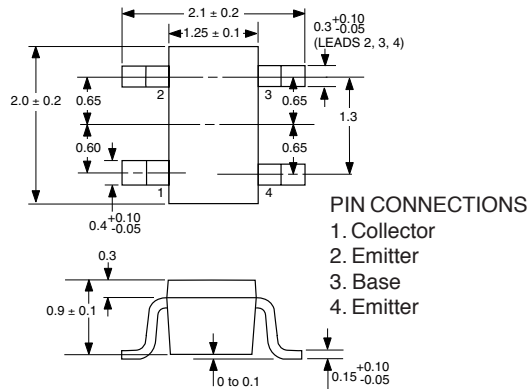
PACKAGE OUTLINE 19
