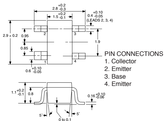
PACKAGE OUTLINE 39R
