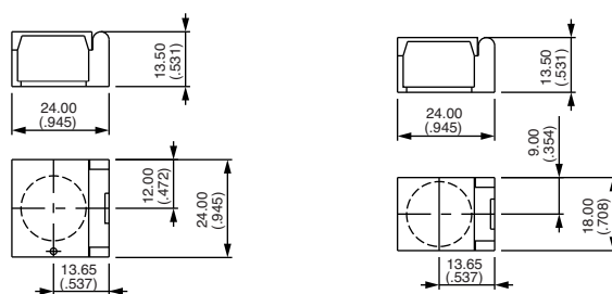
Square/round A01FG2
