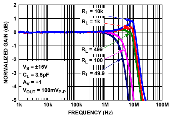
FIGURE 49. CHARACTERIZED CLOSED LOOP GAIN vs R_L
