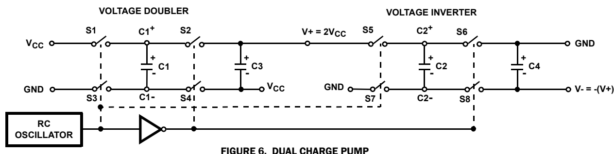
FIGURE 6. DUAL CHARGE PUMP
