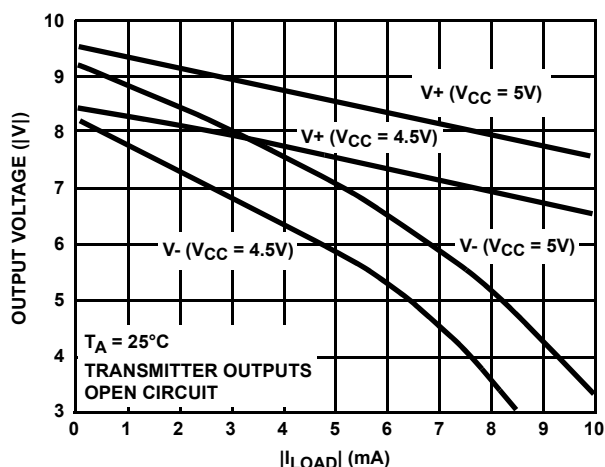
FIGURE 5. V+, V- OUTPUT VOLTAGES vs LOAD CURRENT
