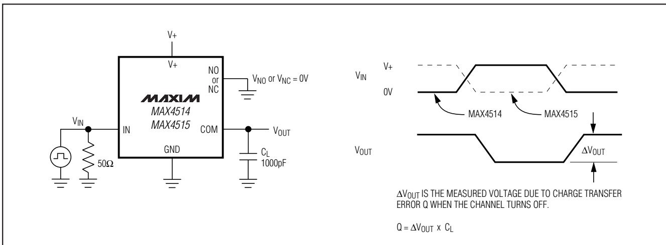
Figure 1. Charge Injection
