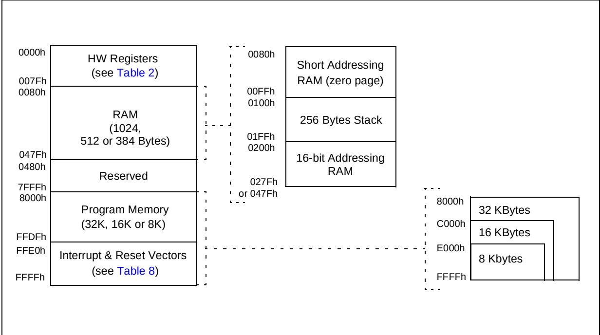
Figure 5. Memory Map
