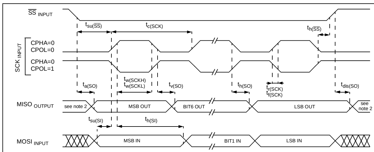
Figure 85. SPI Slave Timing Diagram with CPHA=0 1)
