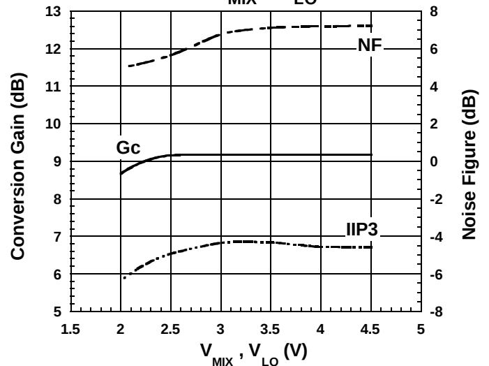
Conversion Gain , Noise Figure , Input-IP3 vs. V_{\text{MIX}} , V_{\text{LO}}
