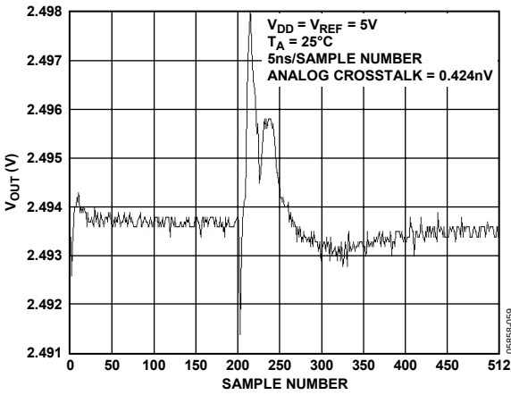
Figure 39. Analog Crosstalk, External Reference
