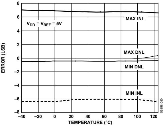
Figure 22. INL Error and DNL Error vs. Temperature
