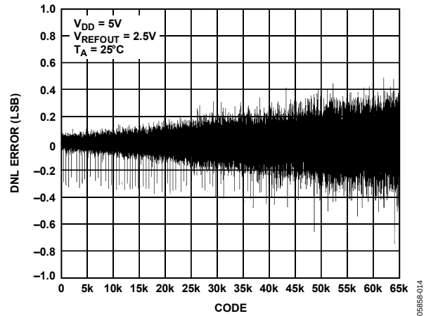
Figure 13. DNL—AD5663R-5
