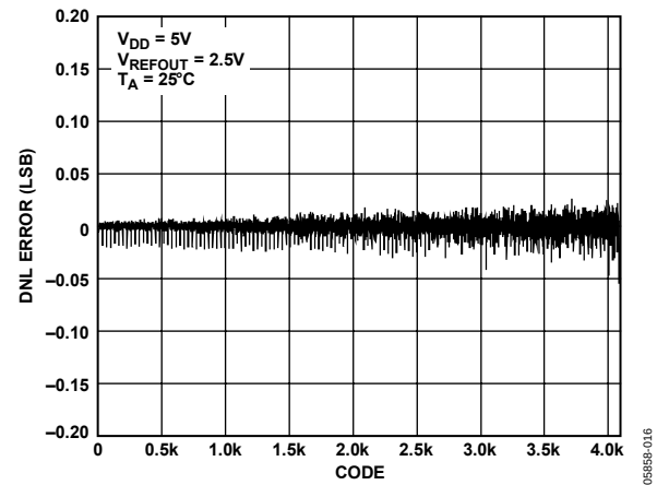
Figure 15. DNL—AD5623R-5
