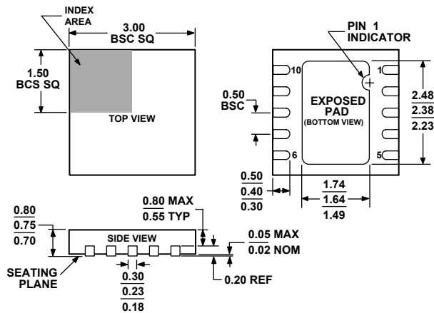
Figure 63. 10-Lead Lead Frame Chip Scale Package [LFCSP_WD] 3 mm x 3 mm Body, Very Very Thin, Dual Lead (CP-10-9) Dimensions shown in millimeters
