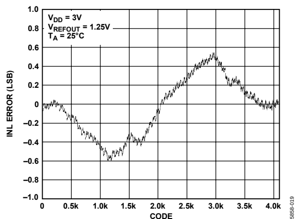
Figure 18. INL—AD5623R-3
