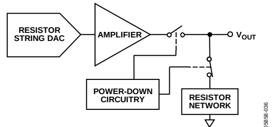
Figure 55. Output Stage During Power-Down
