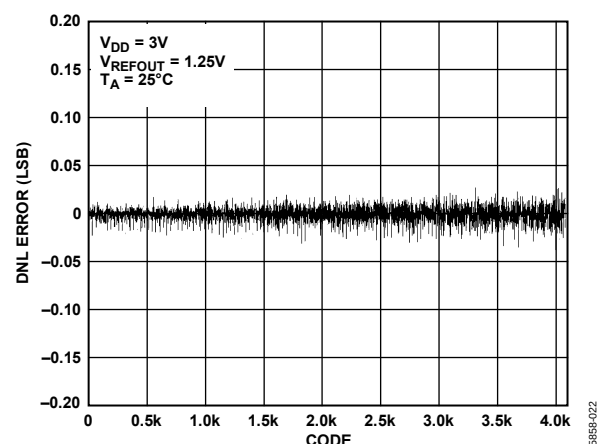
Figure 21. DNL—AD5623R-3
