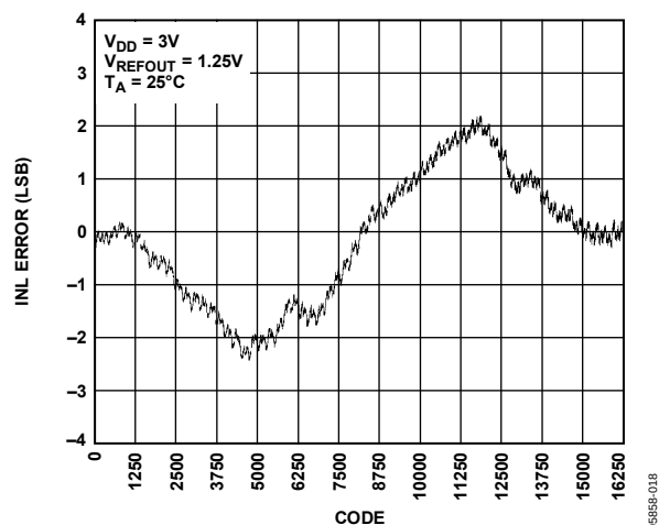
Figure 17. INL—AD5643R-3
