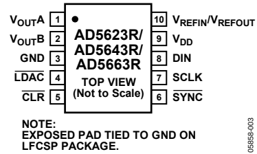
Figure 3. Pin Configuration
