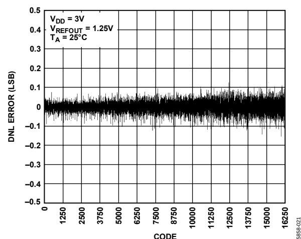
Figure 20. DNL—AD5643R-3
