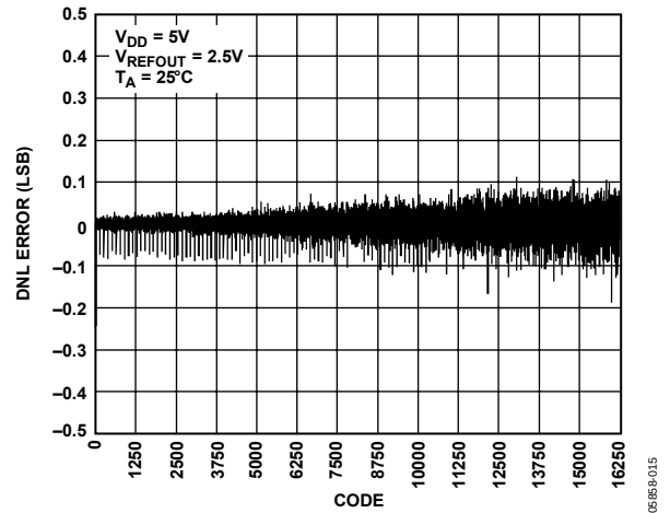
Figure 14. DNL—AD5643R-5
